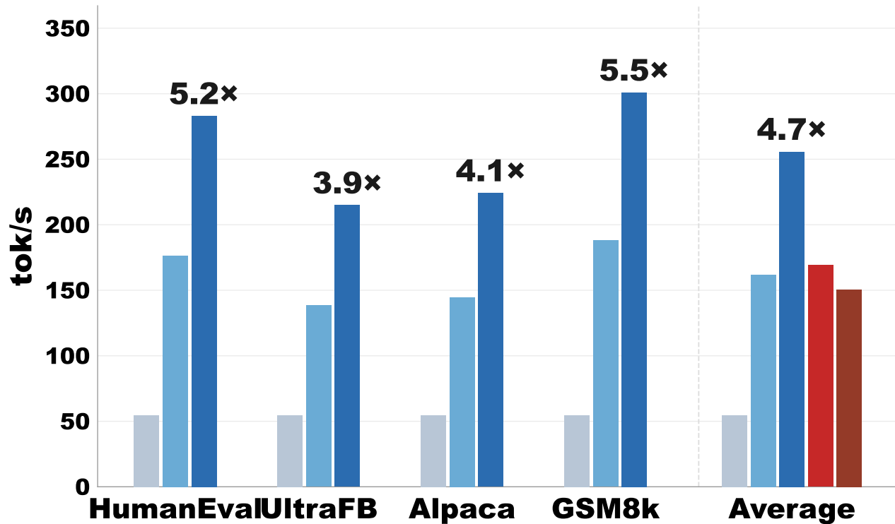
Llama3 End to End Speedups
